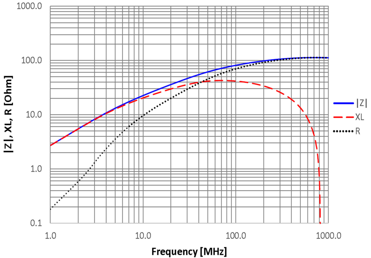
03024-024x / HRB1206S800x1.50x
