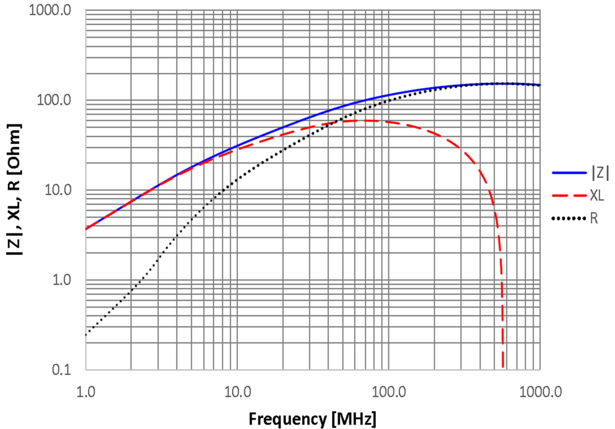
03024-025x / HRB1206S121x1.50x
