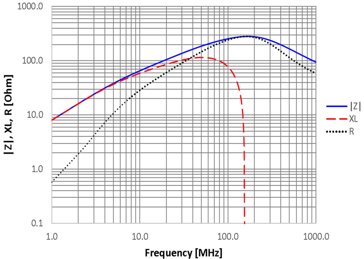
03024-026x / HRB1206S251x1.50x
