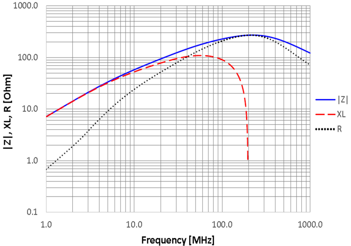
03024-017x / HRB0805S221x1.00x
