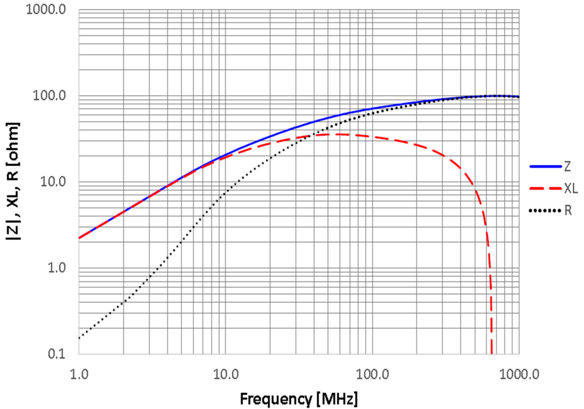
03024-013x / HRB0805S700x1.50x
