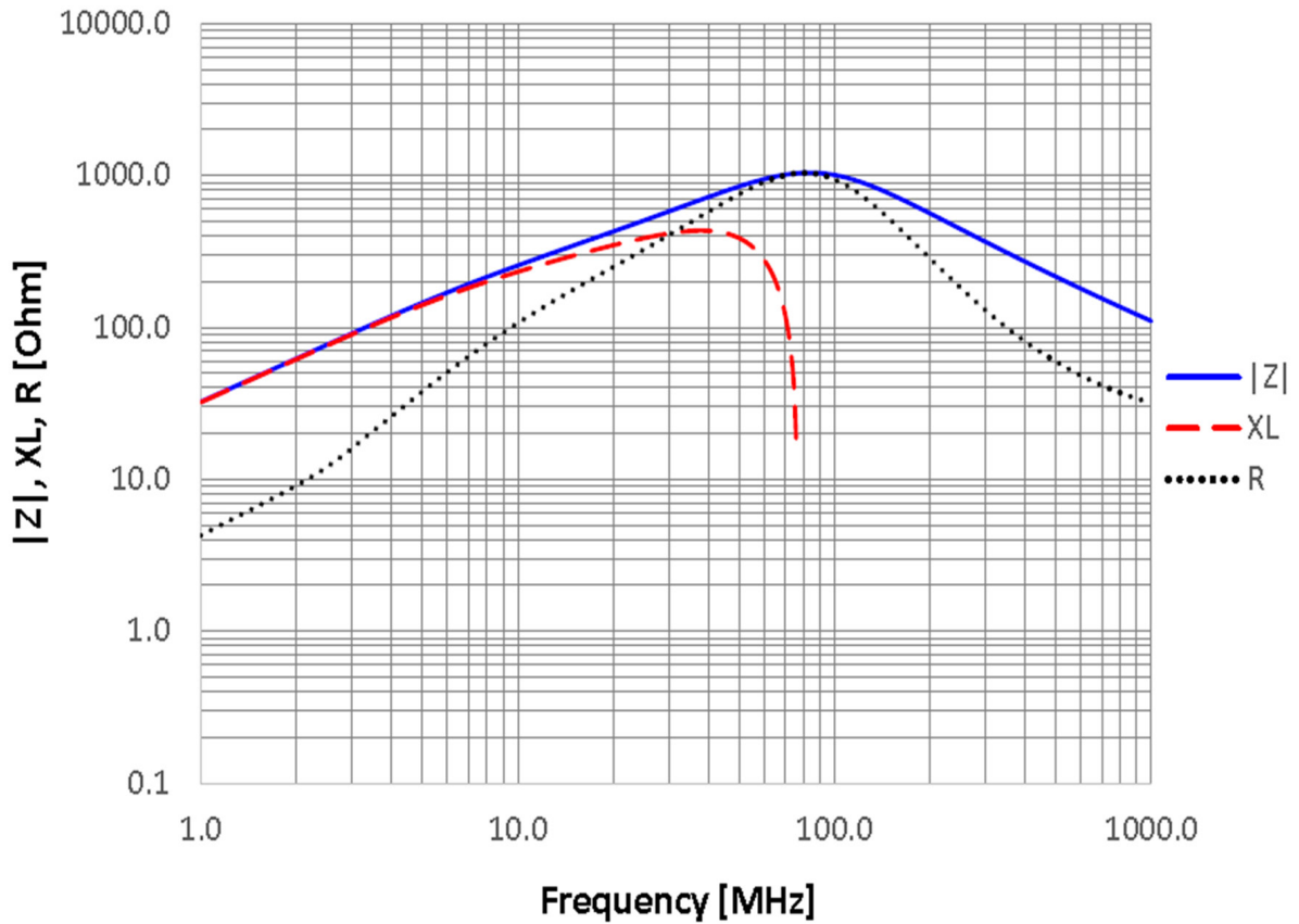
03024-021x / HRB0805S102x1.00x
