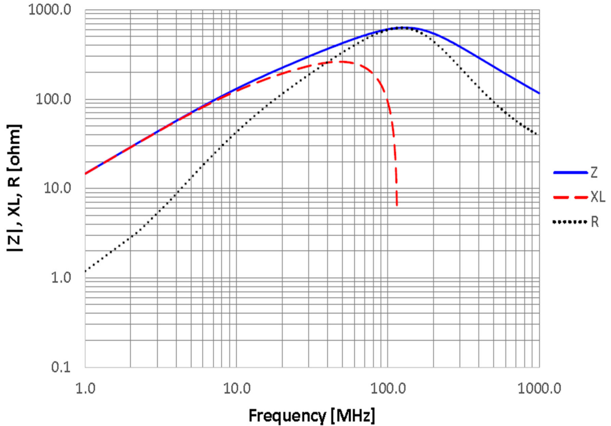
03024-020x / HRB0805S601x1.00x
