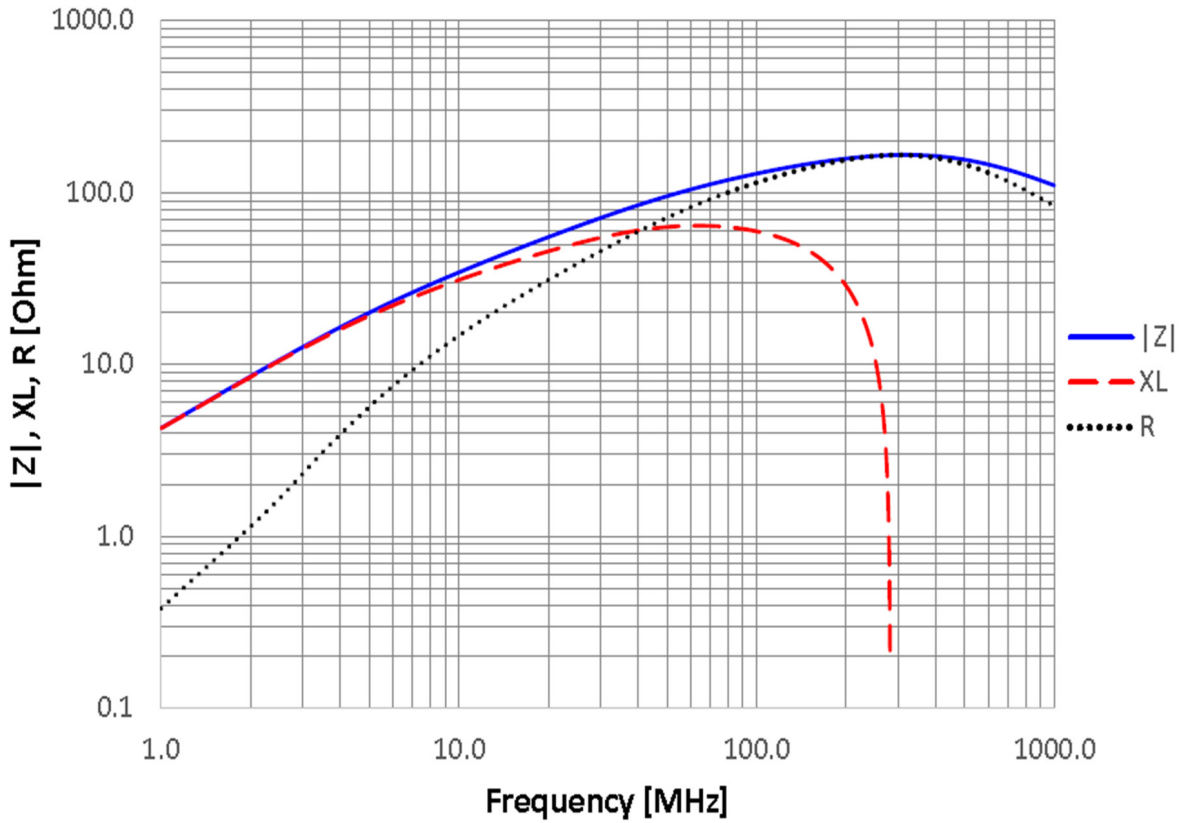
03024-015x / HRB0805S121x1.00x
