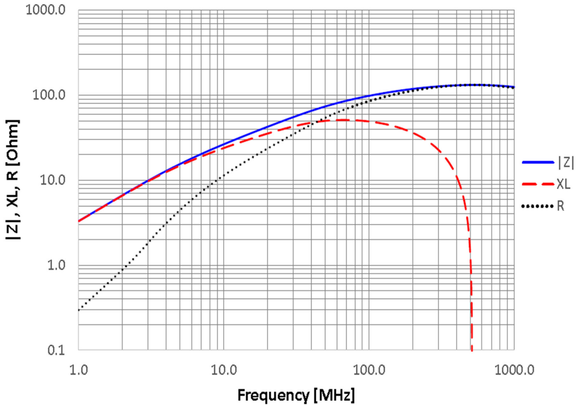
03024-014x / HRB0805S101x1.00x
