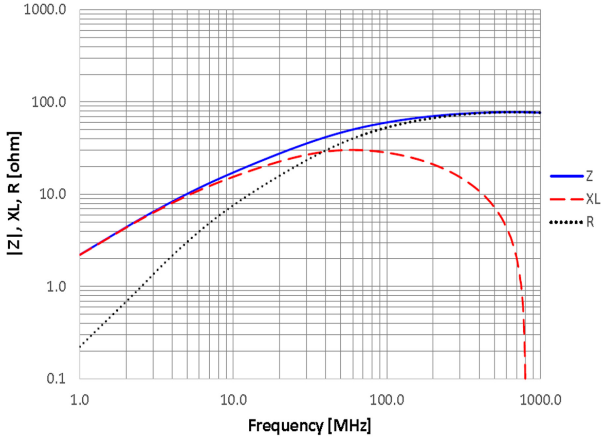
03024-012x / HRB0805S600x1.50x
