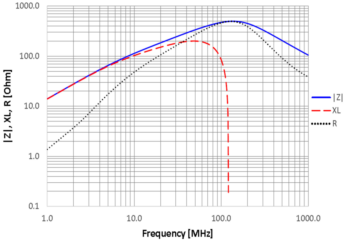
03024-019x / HRB0805S471x1.00x
